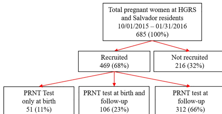
Fig 1. Study flowchart.
